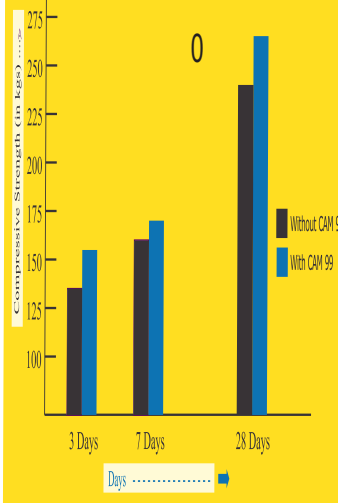
Compressive Strength of concrete without / with CAM-90
